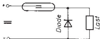
Inductive load (DC)
