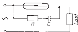
Inductive load
